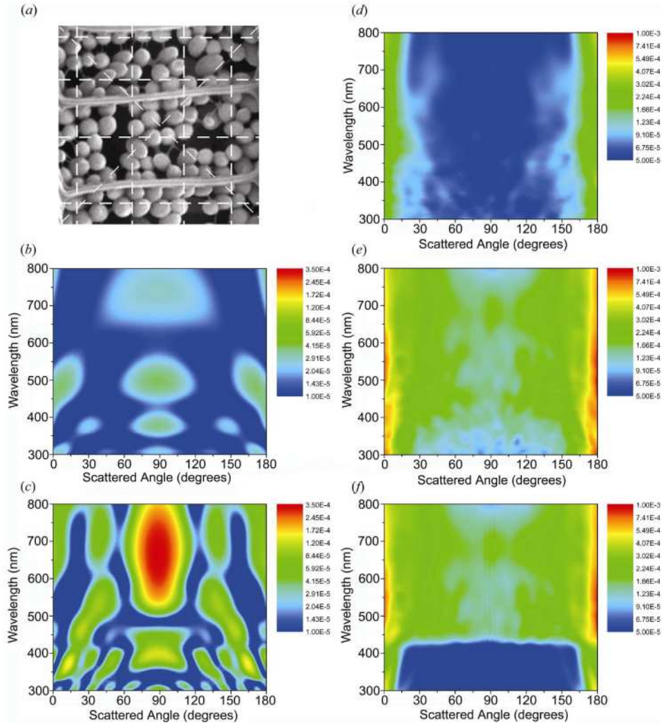
Fig. 3. (a) SEM image of the 2 \mu\text{m} \times 2 \mu\text{m} P. rapae intra-scale region used to generate finite element model geometries. Analysing the position and size of each bead along the ten white dotted lines created ten model scale sections. The power density back scattered into the dorsal hemisphere from each of the ten sections was calculated from the models and a mean average found. The mean scattered power density is plotted in (b) – (f). Initial modelling, (b) and (c), used a single angle of incident at 90^\circ to the scale surface. (b) Scattered power density from a single elliptical bead with a 520 nm long axis and a 170 nm short axis with the long axis parallel to the incident radiation. (c) Scattered power plot when a 95 nm thick substrate is added 800nm below the centre of the single bead described above. This represents the lower substrate of the wing scale. More advance modelling, (d) – (f), used multiple angles of incidence to mimic diffuse illumination (d) Mean back scattered power density plot for the bead array models based described in Fig. 3(a), modelled with no base substrate. (e) Mean back scattered power density plot for the same bead-array models but including the 95 nm thick substrate situated 800 nm below the centre line of the beads. (f) Mean back scattered power density plot for the bead-array models including the base substrate and the UV absorption associated with the pterin pigmentation. Note. (b)-(c) and (d)-(f) are presented with different colour scales.
